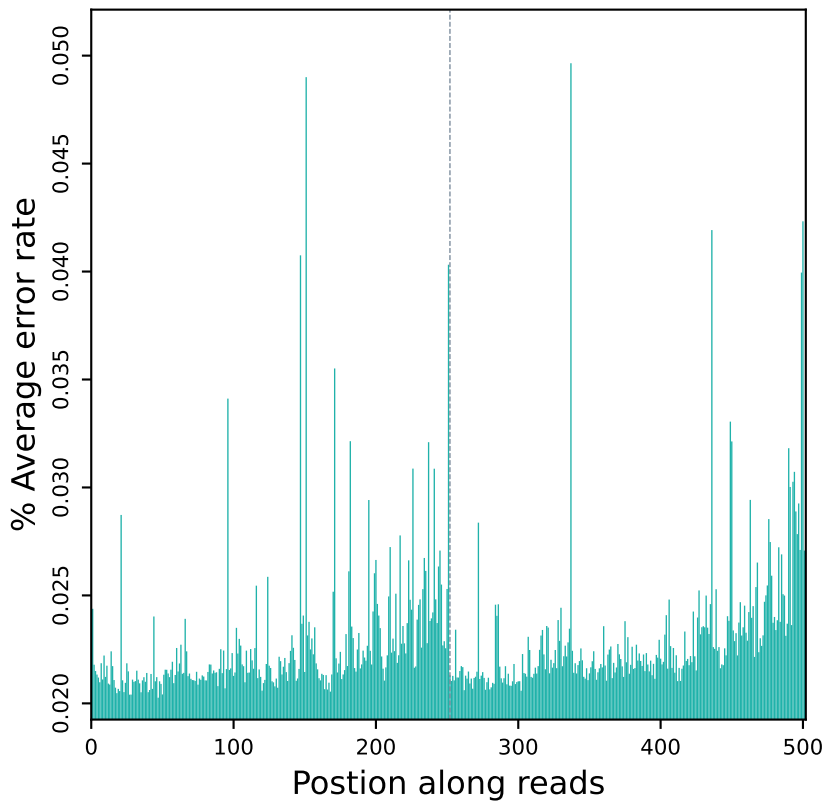
Error rate distribution along reads (R10402)
